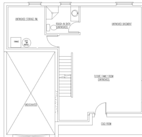
BASEMENT / FOUNDATION PLAN
