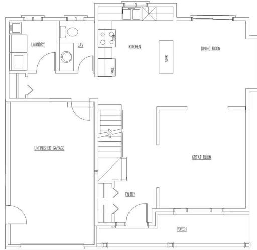
MAIN LEVEL FLOOR PLAN - 813 sq.ft. FINISHED LIVING AREA GARAGE AREA- 269 SQ. FT.
