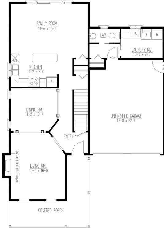
MAIN LEVEL FLOOR PLAN 1028.5 SQ. FT. FINISHED FLOOR AREA 465 SQ. FT. GARAGE AREA
