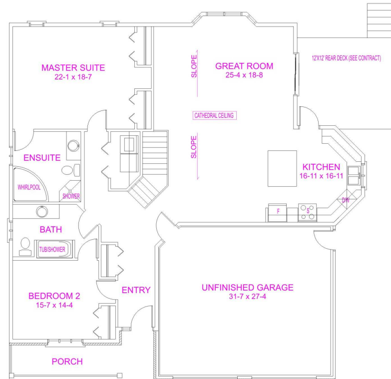
MAIN LEVEL FLOOR PLAN 1606 SQ. FT FINISHED LIVING AREA 534.6 SQ. FT GARAGE AREA
