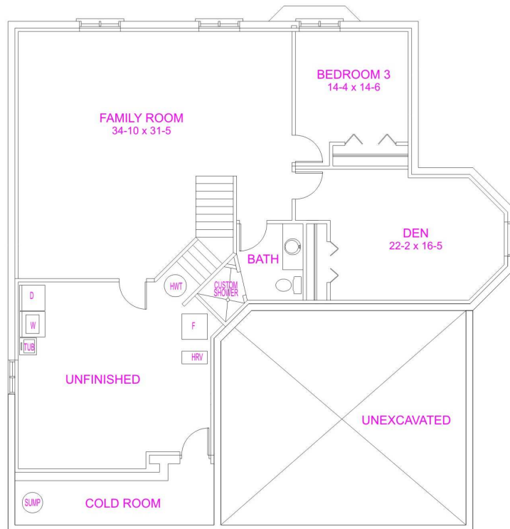
BASEMENT PLAN FINISHED FLOOR AREA= 1117 SQ. FT.
